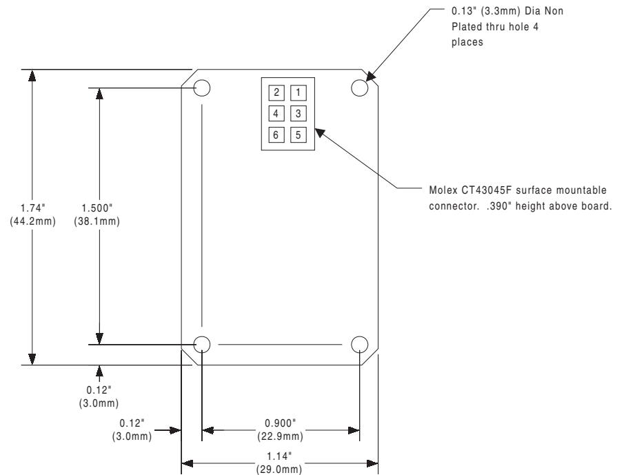
Figure 2. Mechanical Drawing
