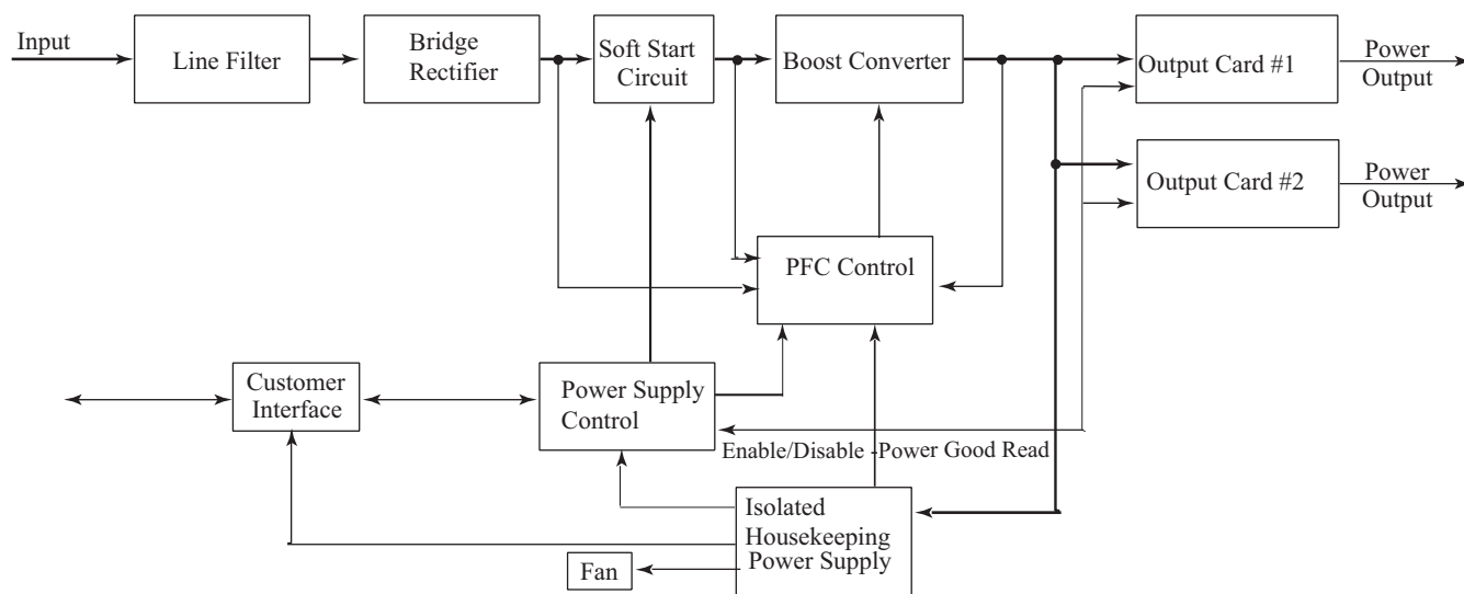
Figure 1. PFC Micro Architecture
