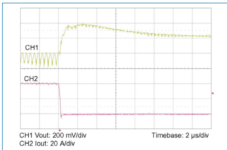
Figure 11 — 40-0 A load step with 100 \mu F input capacitor and no output capacitor.
