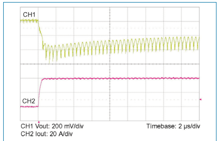
Figure 10 — 0-40 A load step with 100 \mu F input capacitor and no output capacitor.
