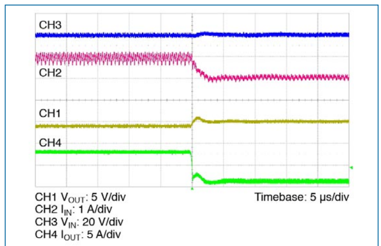
Figure 12 — Negative load transient (7.3 A – 0 A)
