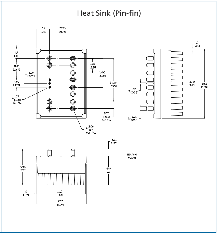
Figure 17 — Pin-fin heat sink outline
