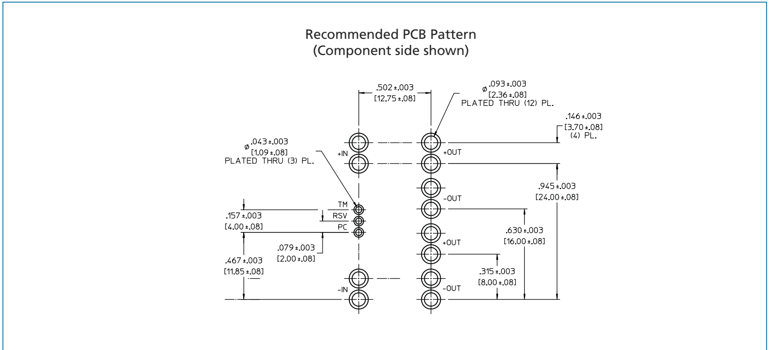
Figure 18 — PCB mounting specifications
