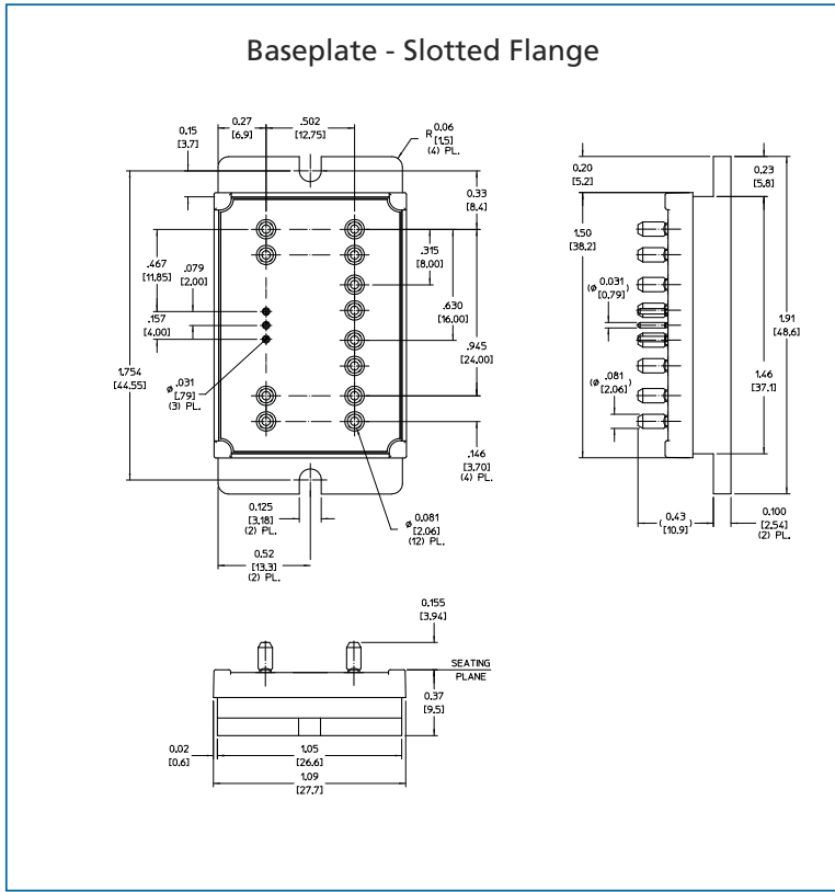
Figure 16 — Module outline
