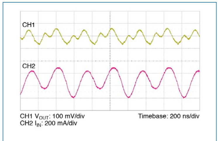
Figure 10 — Output voltage and input current ripple, 270 V_{in} , 235 W no C_{OUT}
