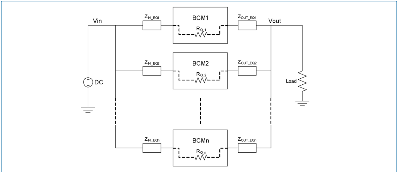
Figure 21 – BCM Array
