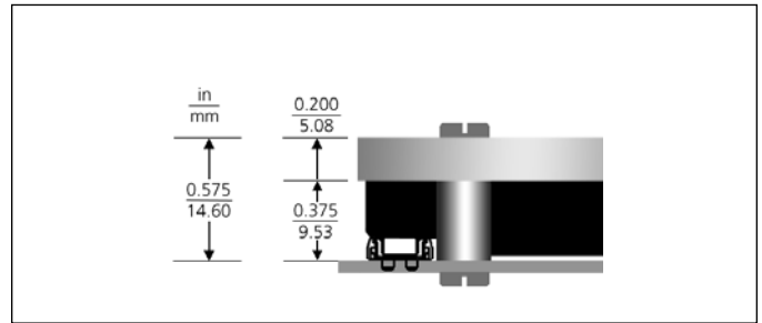
Figure 17-4 — Through-hole or threaded baseplate; Height above board with standoff
