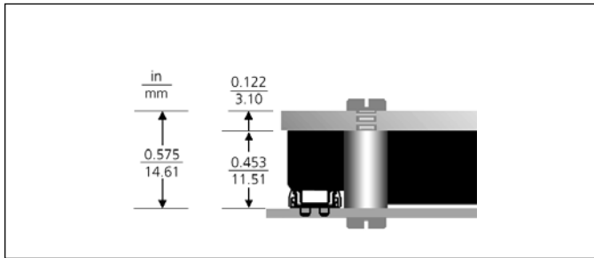
Figure 17-3 — Slotted baseplate; Height above board with standoff
